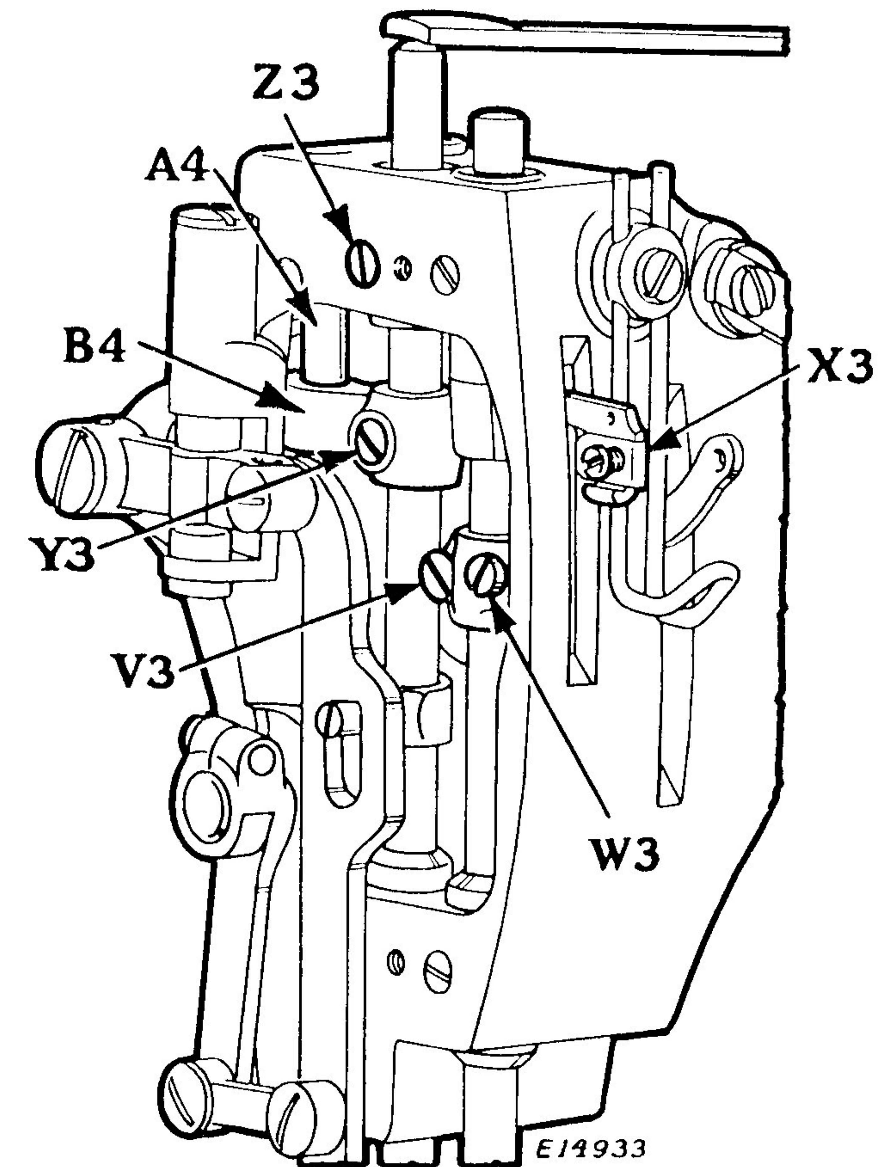
Fig. 14. Setting Needle Bar, and Other Adjustments
