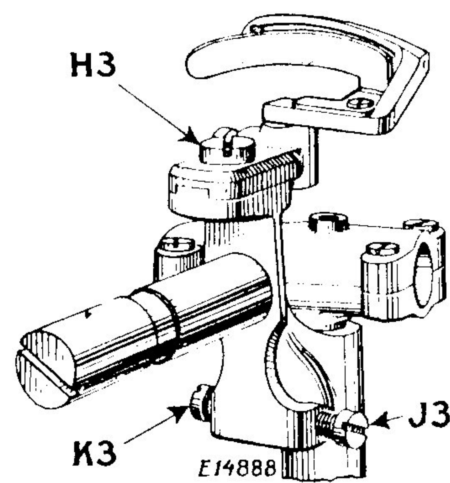
Fig. 12. Setting the Looper Machine 147-88
