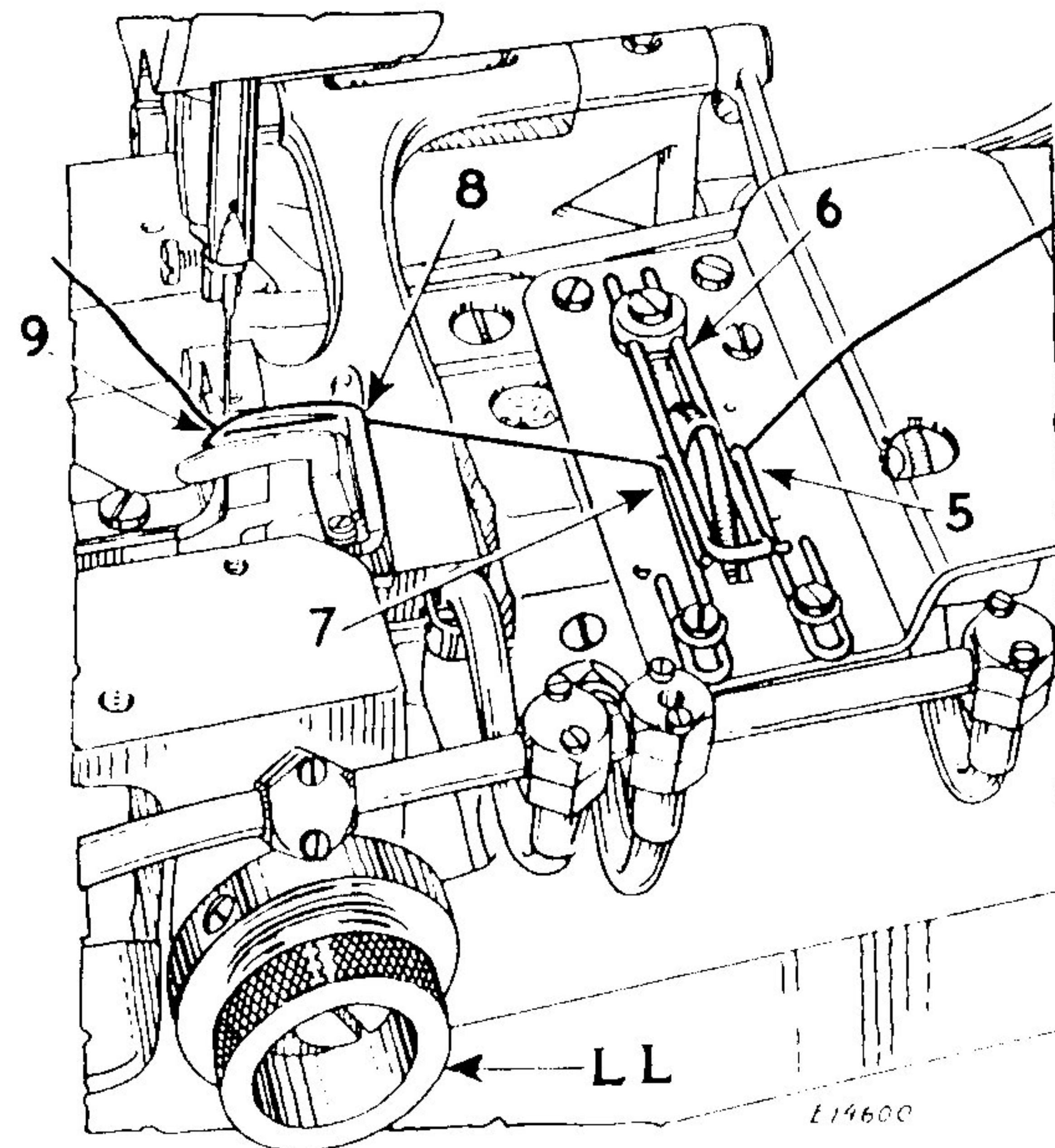
Fig. 7. Threading the Looper on Machine 147-83
