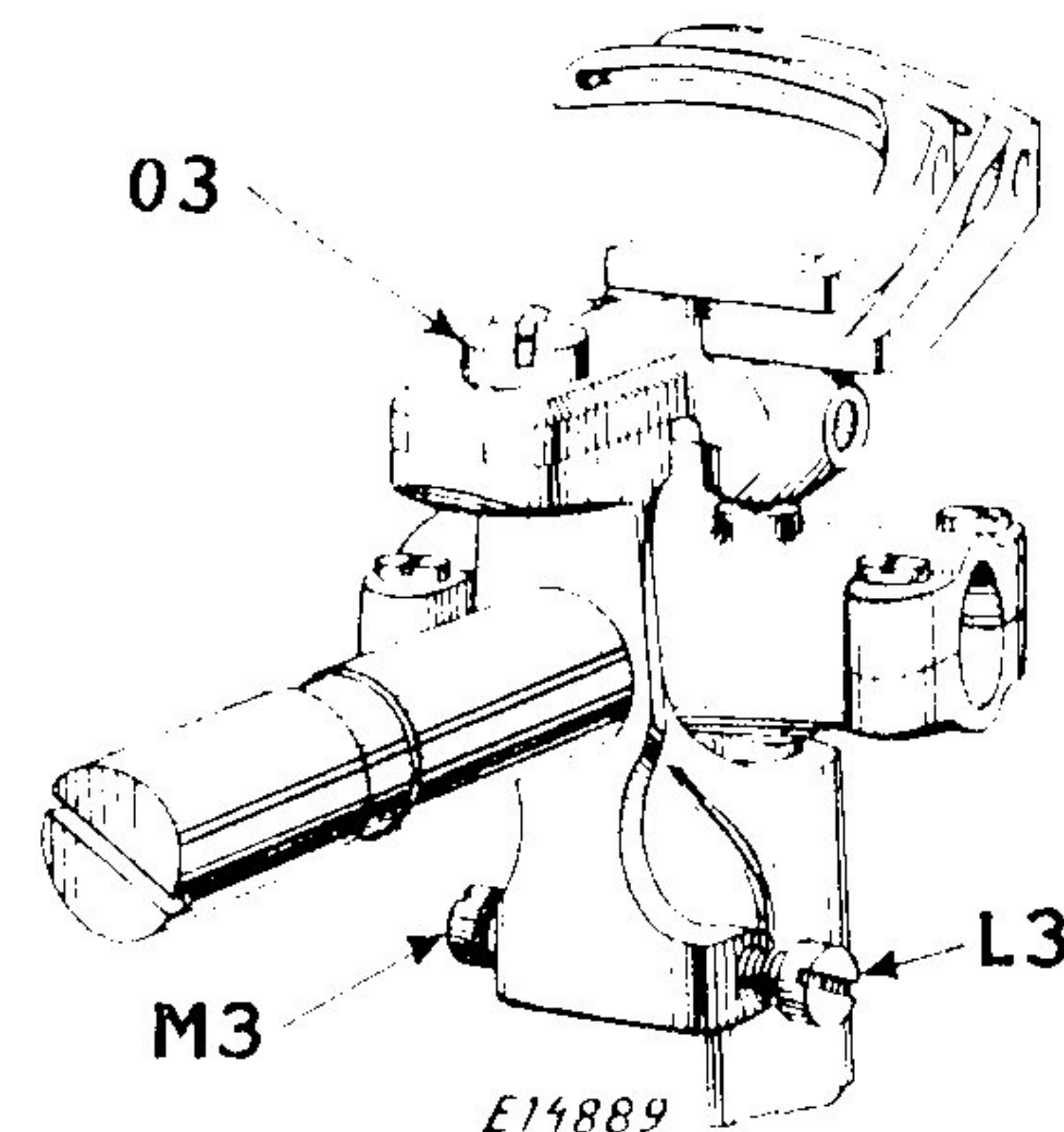
Fig. 13. Setting the Loopers Machines 147-110 and 147-111
