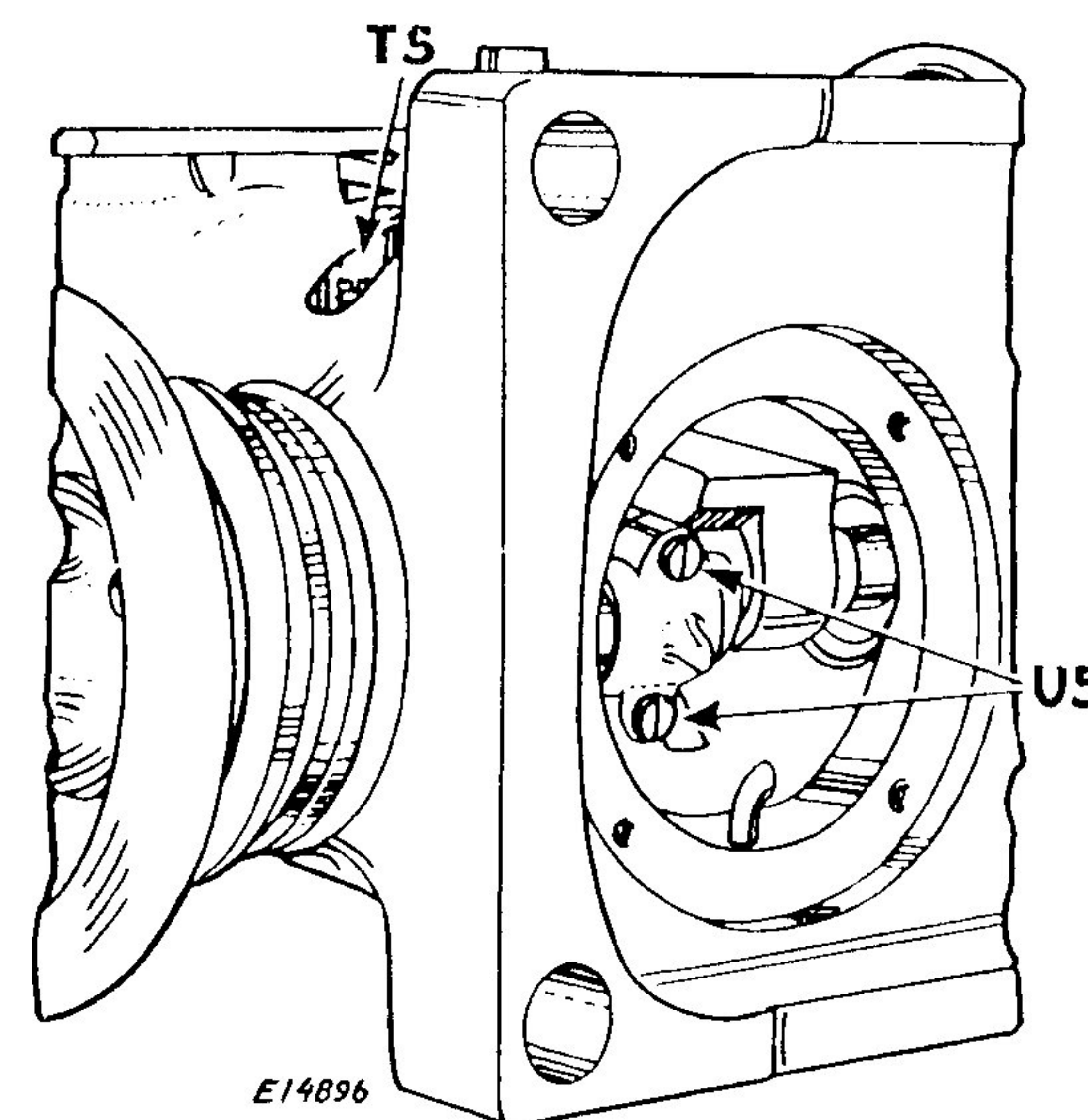
Fig. 24. To Remove Arm Rotary Shaft
