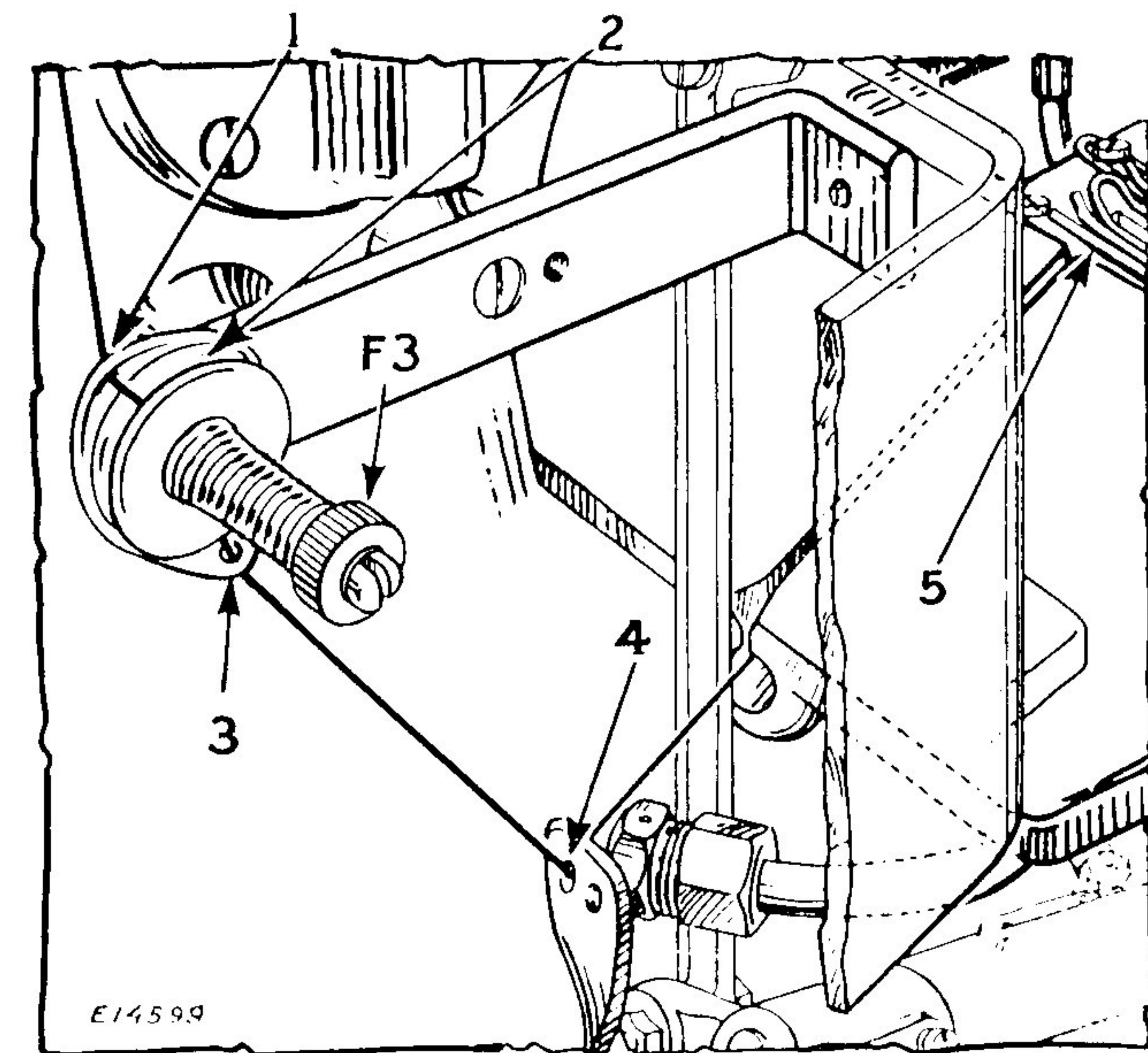
Fig. 6. Threading the Loper on Machine 147-88
