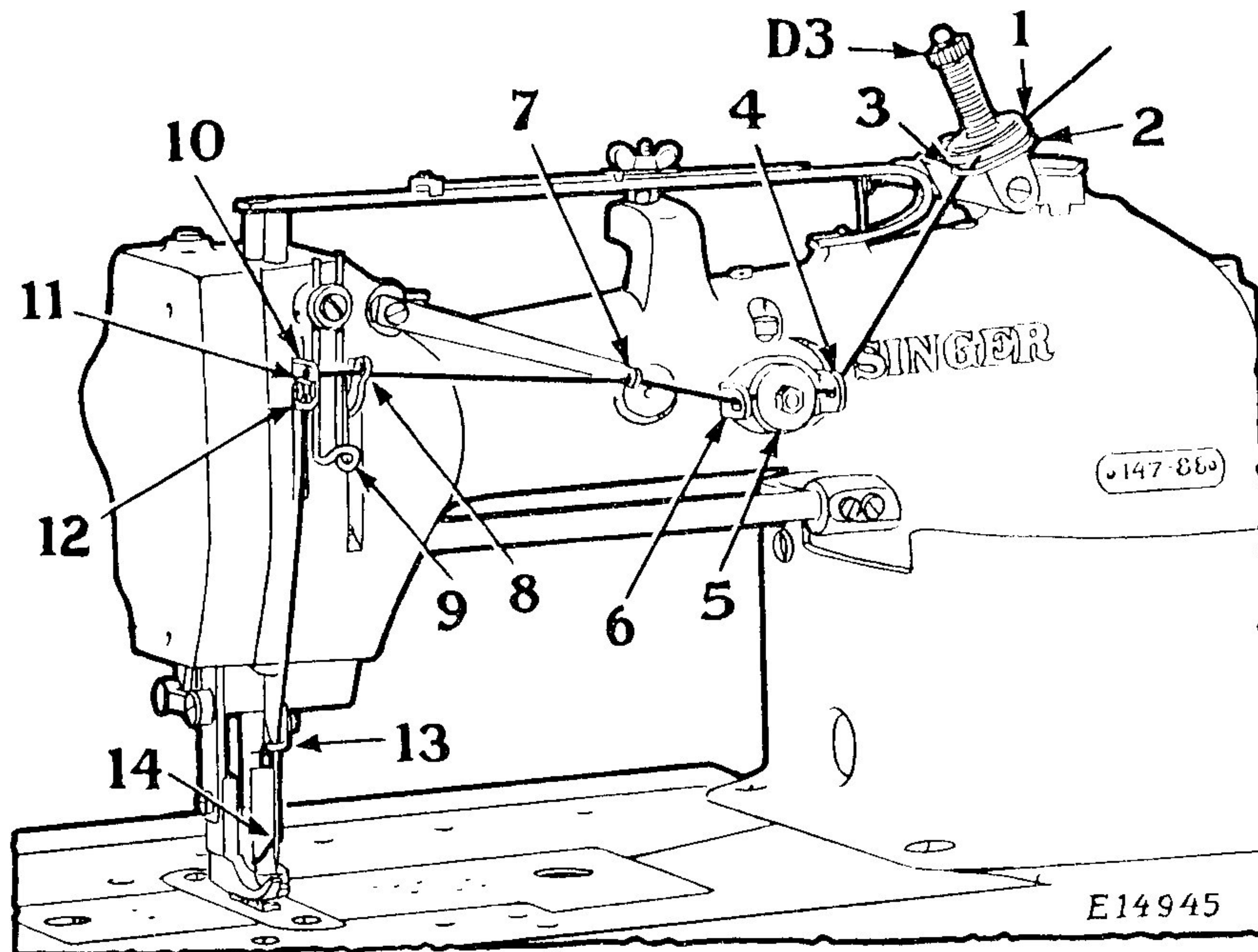
Fig. 5. Threading the Needle, Machine 147-88
