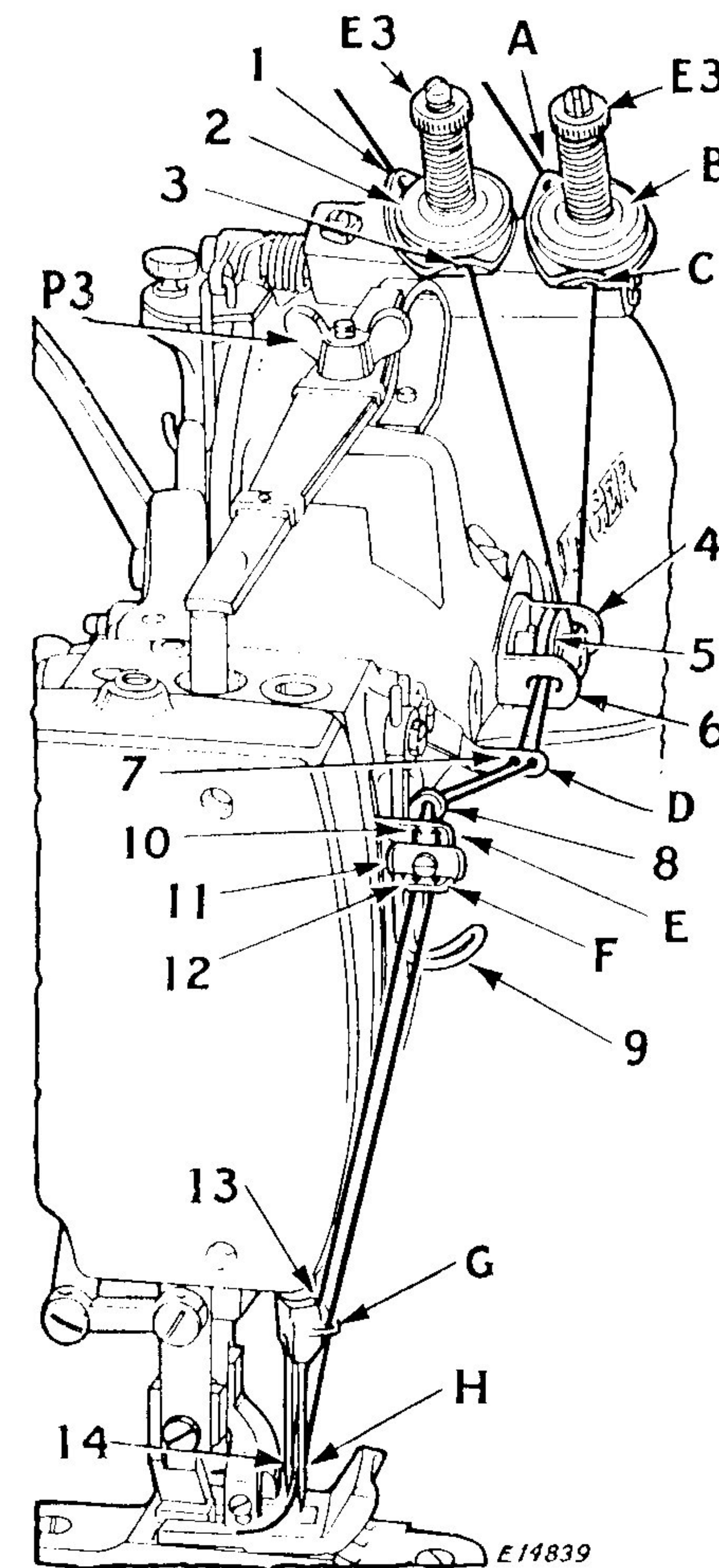
Fig. 8. Threading the Needles Machines 147-110 and 147-111
