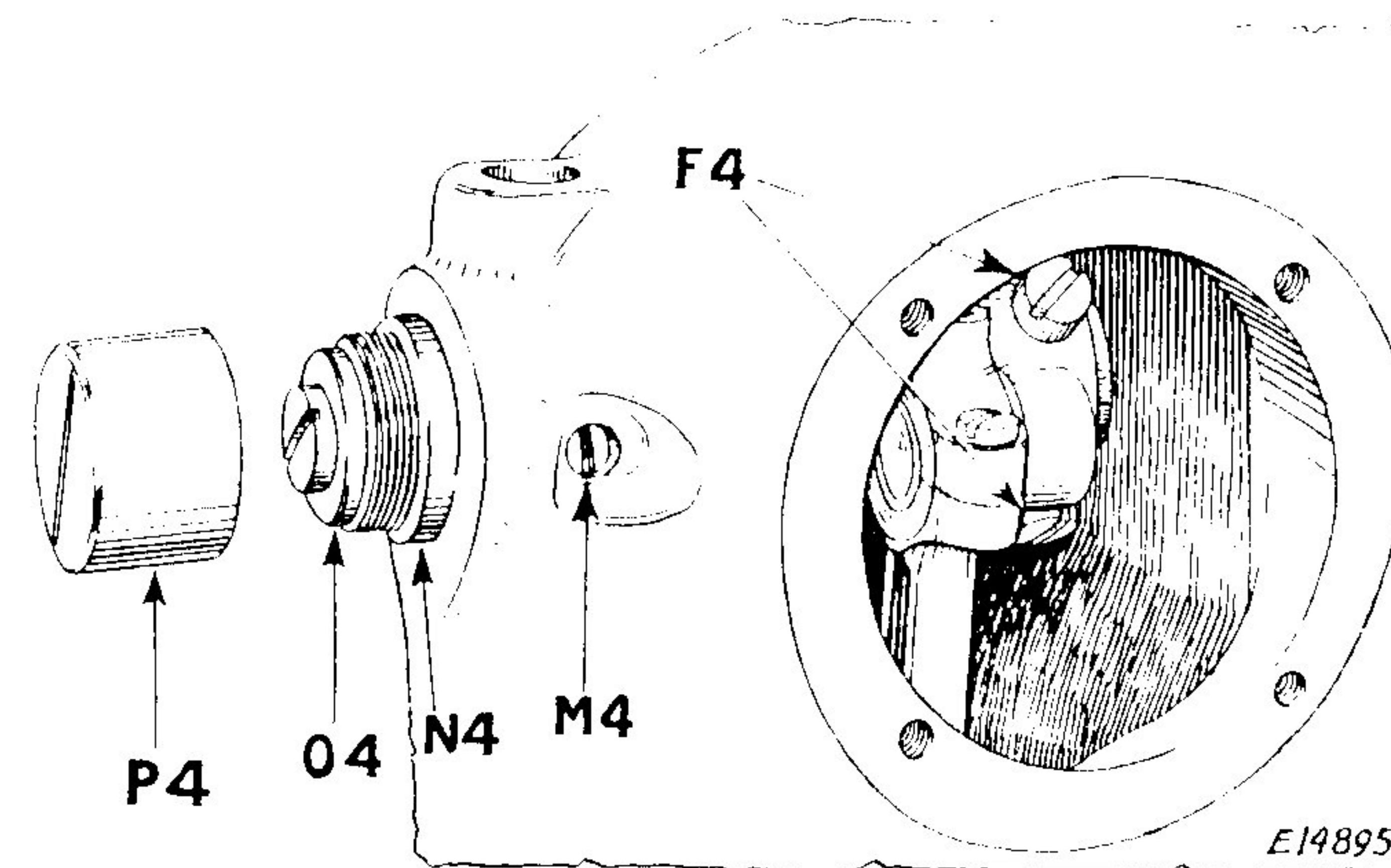
Fig. 19. Removing the Arm Rock Shaft
