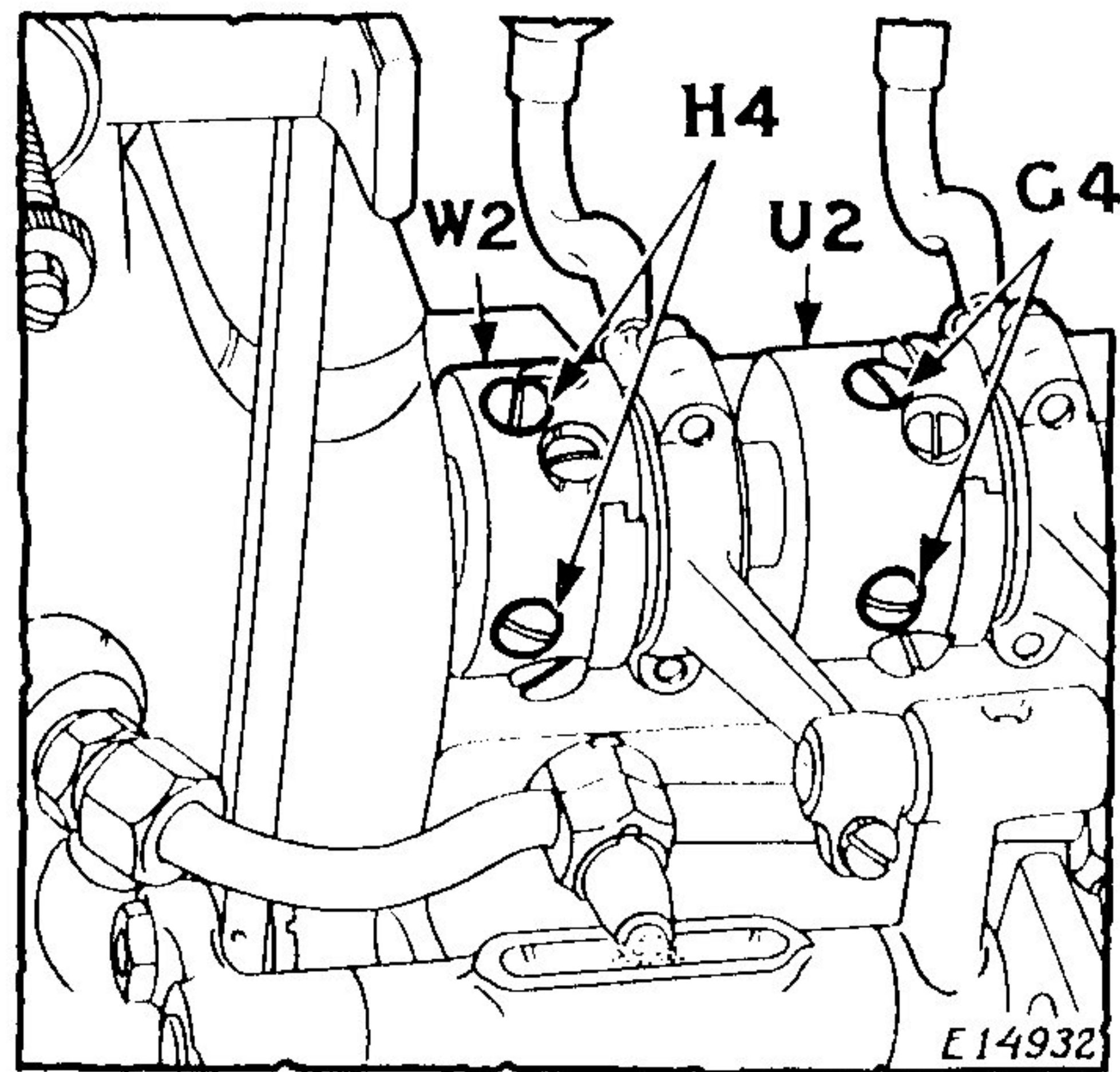
Fig. 17. To Regulate Sidewise Movement of the Loopers
