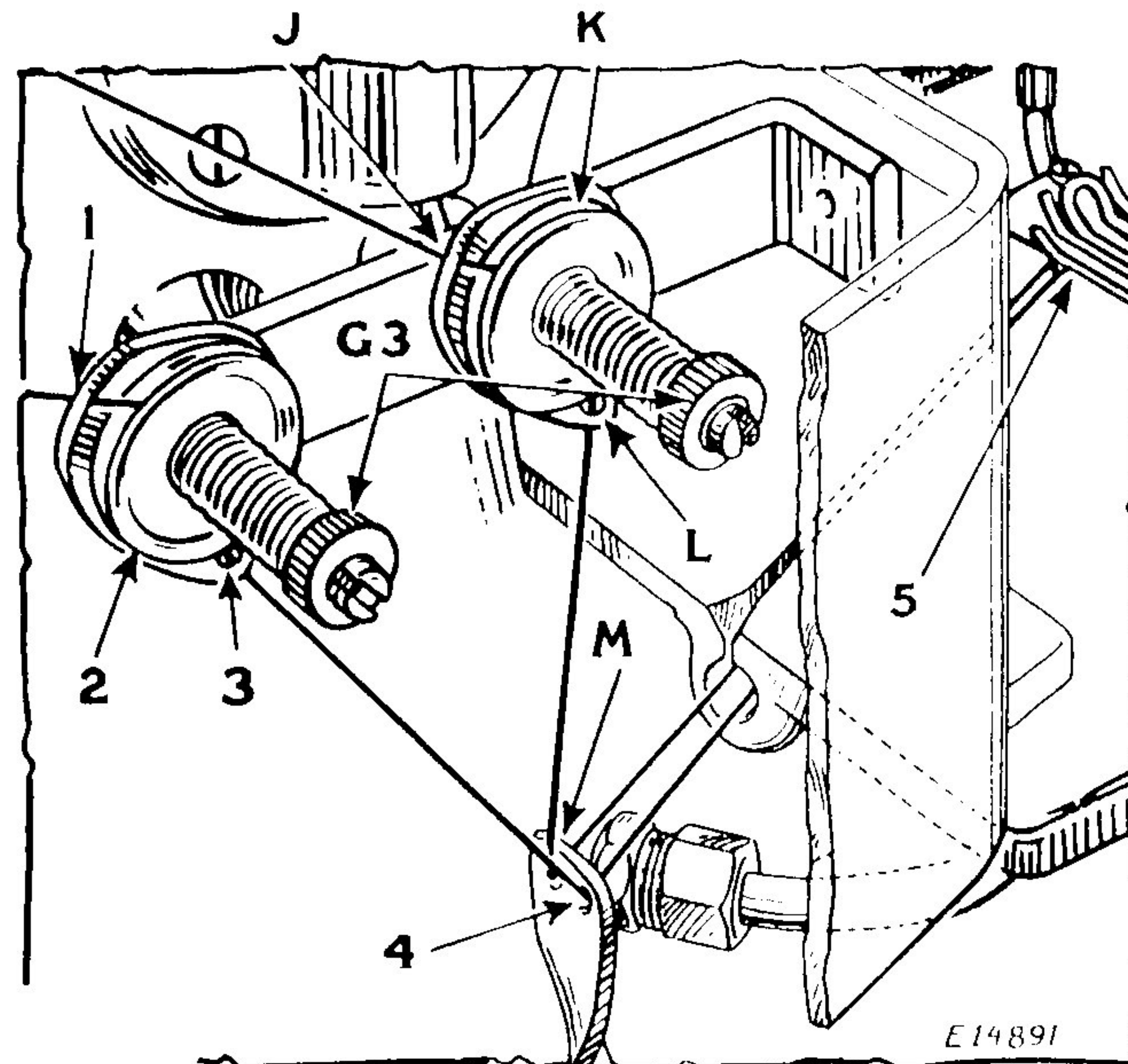
Fig. 9. Threading the Loopers on Machines 147-110 and 147-111
