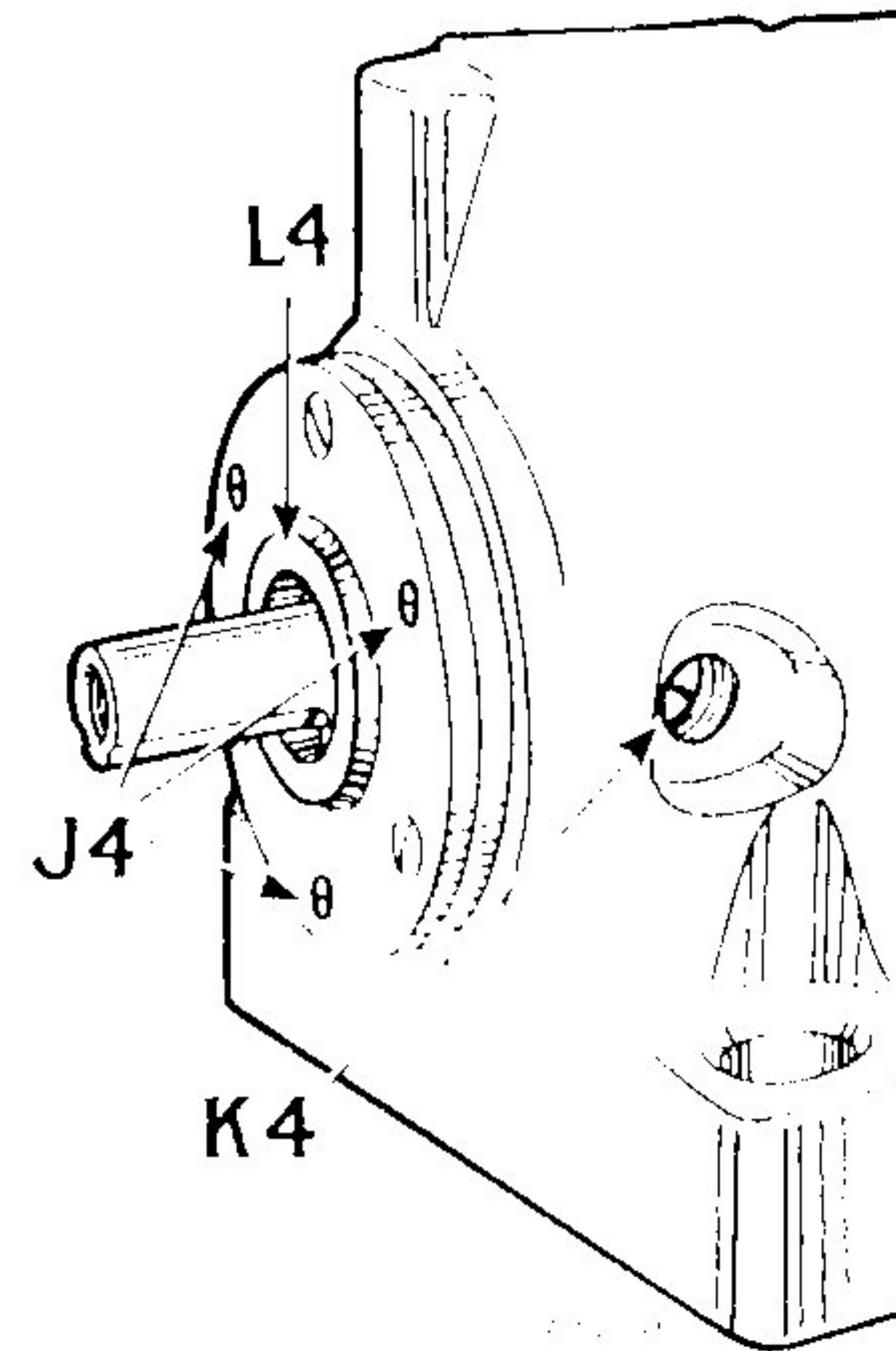
Fig. 17. To Regulate Sidewise Movement of the Loopers
