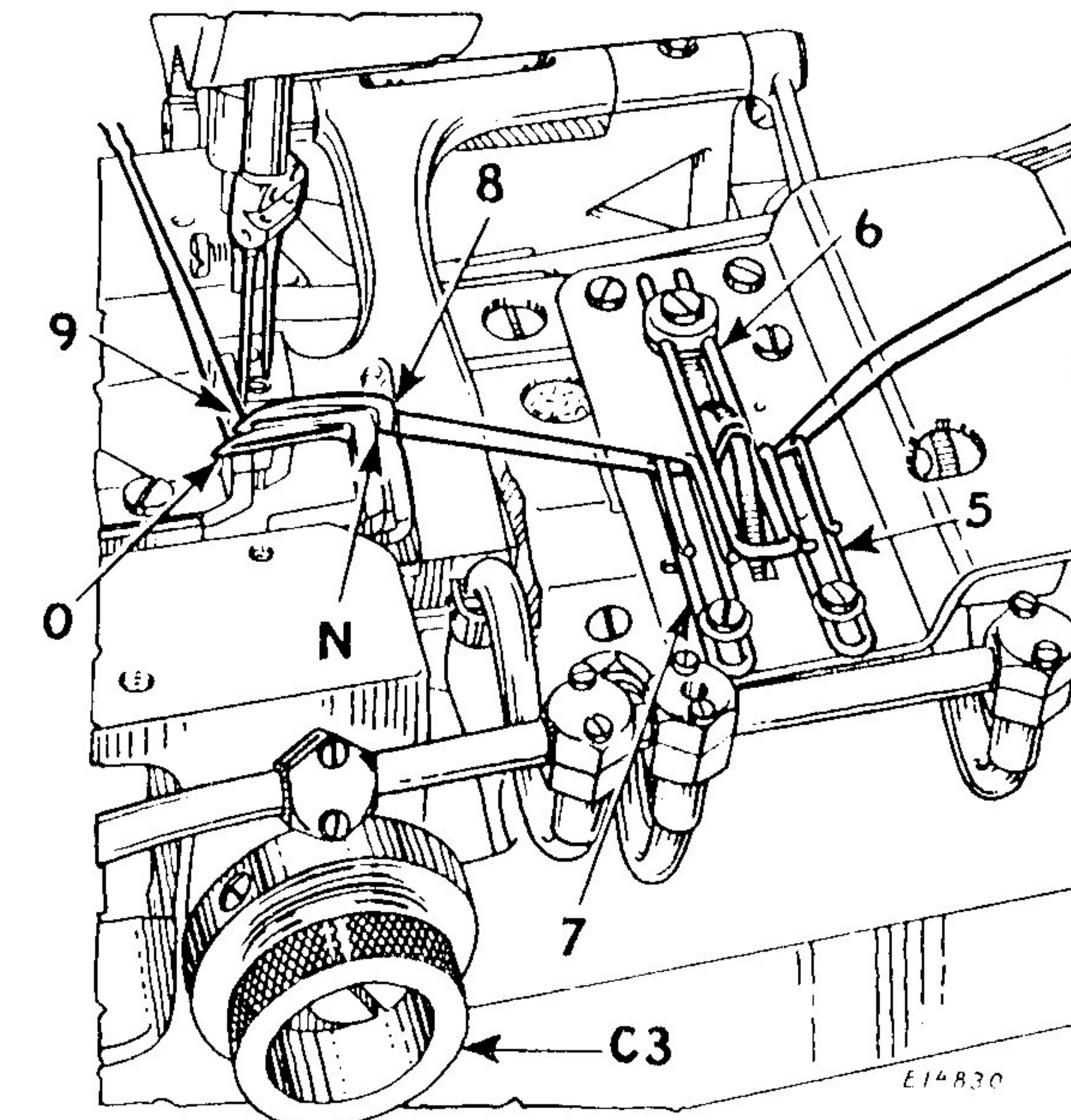
Fig. 10. Threading the Loopers on Machines 147-110 and 147-111
