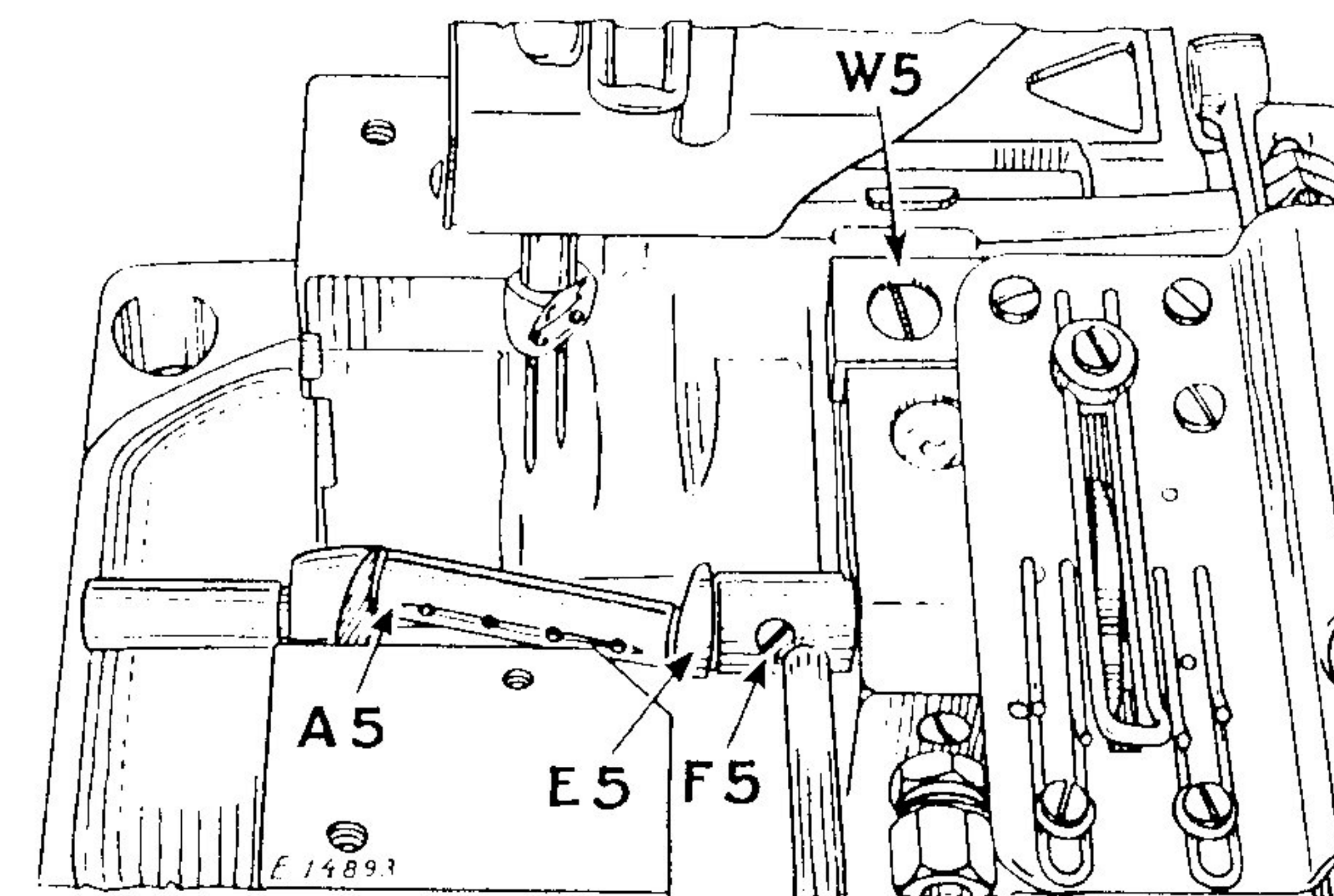
Fig. 22. To Remove the Loper Shaft
