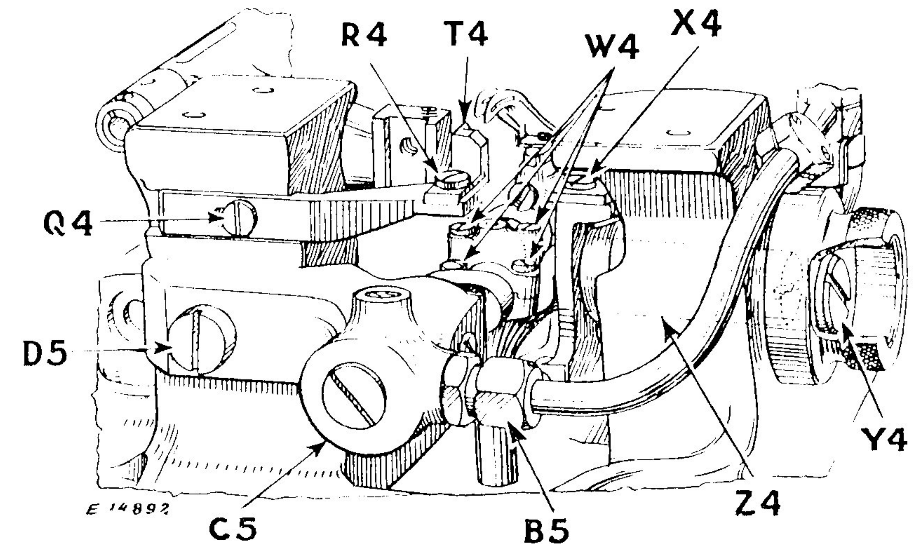
Fig. 21. To Remove the Loper Mechanism
