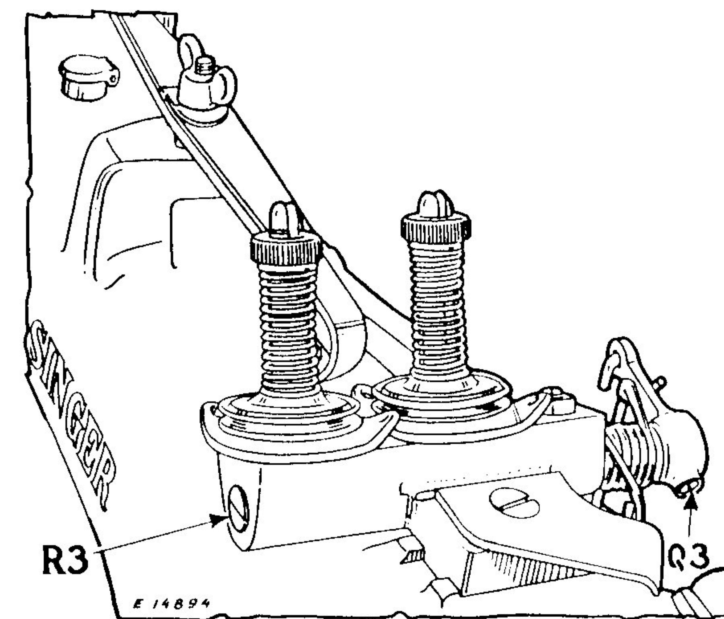
Fig. 16. Adjustment of Thread Tension Releaser
